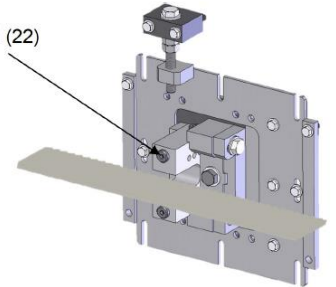
Support for band saw with short nozzle head
