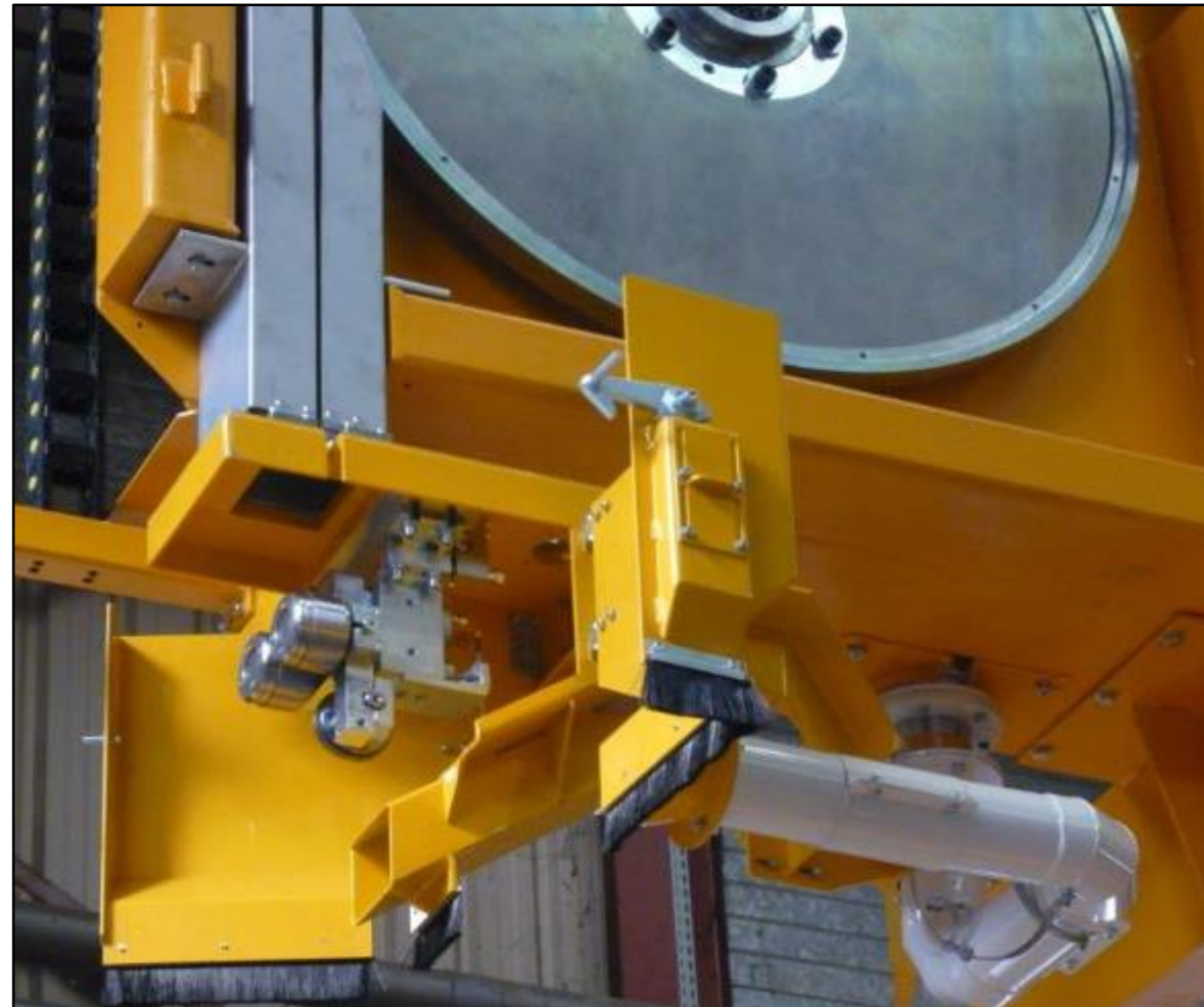
Blade-guide rollers
